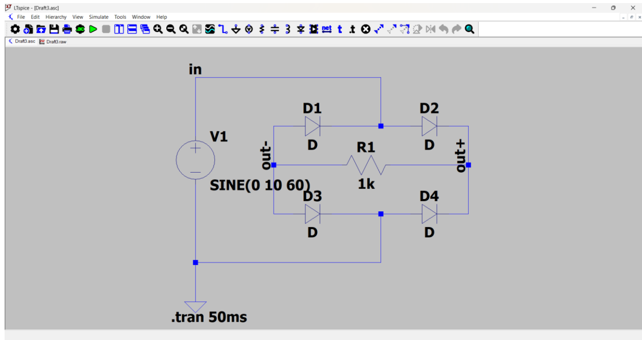
Screenshot 1: LTspice Schematic window
